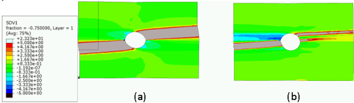
Figure 23. Failure of OHC cross-ply specimen due to kink band formation. a) AS4/EPON862 system with 56% volume fraction of AS4. b) AS4/C-300/EPON862 system with 56% volume fraction of AS4 and 1.21% volume fraction of GNP within EPON862 matrix.
