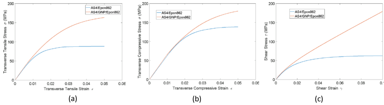
Figure 21. Comparison of stress-strain response of AS4/EPON862 composite ply with 56% volume fraction of AS4 and AS4/GNP/EPON862 composite ply with 56% volume fraction of AS4 and 1.21% volume fraction of GNP within EPON862 matrix. a) Transverse tension. b) Transverse compression. c) Shear.
