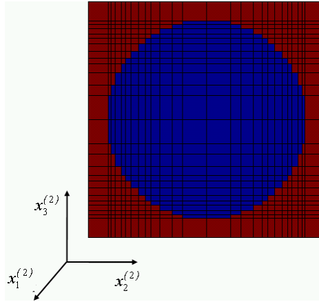
Figure 7. Level 2 MAC/GMC GNP/epoxy RUC containing lastic subcells with CF (blue), and subcells representing epoxy with randomly oriented GNPs (red) modeled with.
