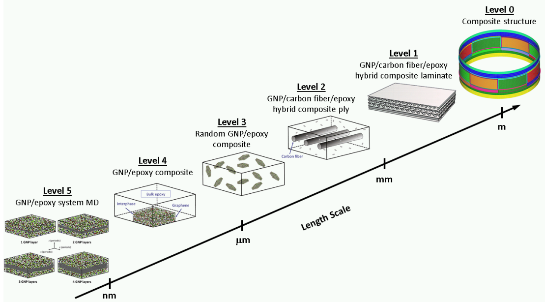
Figure 2: Multiscale modeling hierarchy. Level 5: Nanoscale. Level 4: Nanoscale Continuum. Level 3: Microscale Matrix. Level 2: Lamina Scale. Level 1: Laminar Scale. Level 0: Structural Scale.
