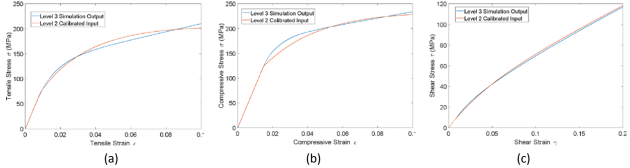
Figure 15: Results from Level 3 simulation of randomly oriented GNP within EPON862 compared to calibrated MMCDM input for homogenized GNP/EPON862 subcells at Level 2. a) Tension. b) Compression. c) Shear.
