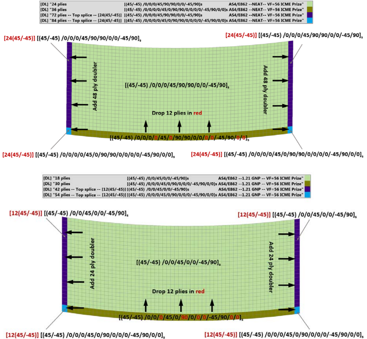
Figure 29: Details of the panel top facesheet layups and ply transitions for a one-eighth circumferential section of the CEUS composite panel designs for (a) the neat epoxy matrix material system and (b) the GNP enhanced matrix system.
