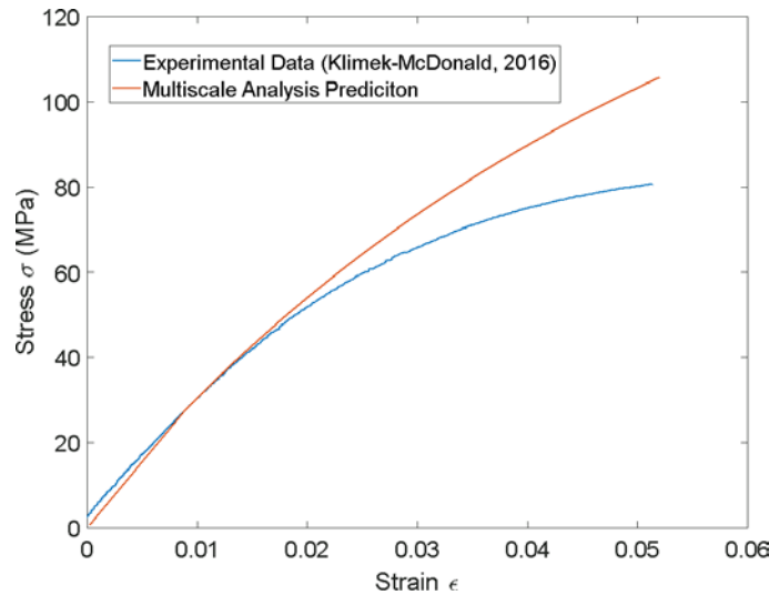
Figure 16: Level 3 prediction of non-linear tensile stress strain response of EPON862 epoxy with 1.21% GNP volume fraction compared to experimental data.
