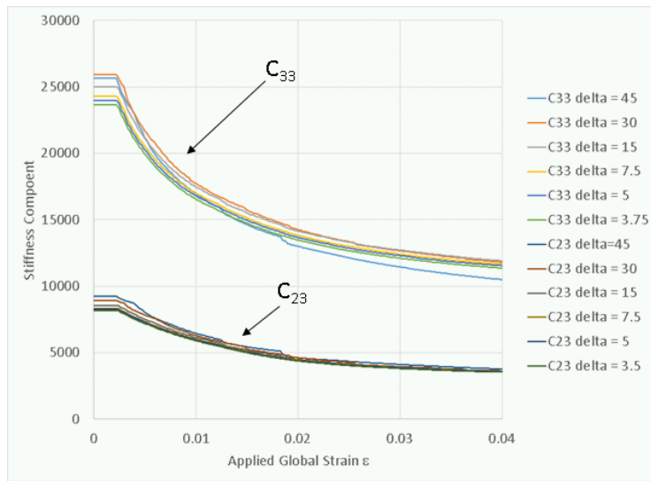
Figure 30. Evolution of nonlinear stiffness components C_{33} and C_{23} calculated using Eqs. (6) and (7) for a range of orientation angle increments \Delta\theta , \Delta\phi (delta).
