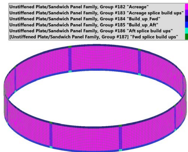
Figure 10. Sizing groups, which have been required to have the same design, employed in the sizing process.
