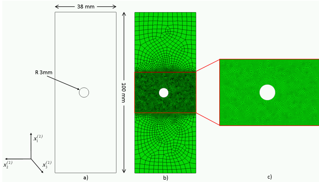
Figure 8: OHC FEM model. a) Geometry of OHC specimen based on ASTM Standard D 6484/D 6484M. b) FEM mesh. c) Exploded view of refined FEM mesh in gage section.
