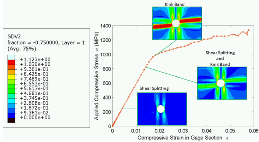
Figure 25. Damage progression predicted with ST in OHC cross-ply specimen composed of AS4/C-300/EPON862 system with 56% volume fraction of AS4 and 1.21% volume fraction of C-300 within EPON862 matrix.
