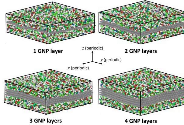
Figure 5. Equilibrated MD models for varying number of graphene layers.
