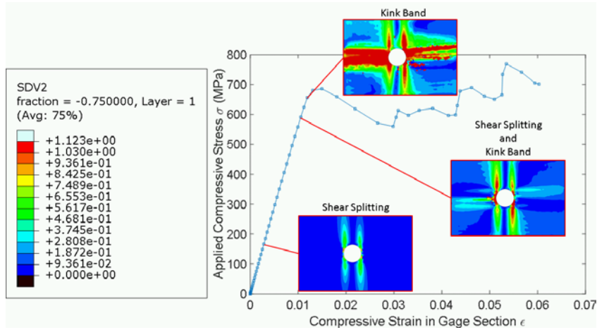
Figure 24. Damage progression predicted with ST in OHC cross-ply specimen composed of AS4/EPON862 system with 56% volume fraction of AS4.
