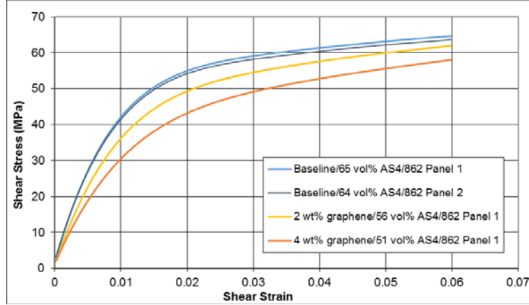
Figure 13: Average stress-strain curves for shear tests up to 0.06 strain. Graphene content is reported as weight percent in epoxy. Carbon fiber content is reported as volume percent in composite.
