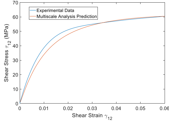
Figure 17: Level 2 prediction of nonlinear shear stress-strain response of AS4/EPON862 with 64.8% AS4 volume fraction compared to experimental data.
