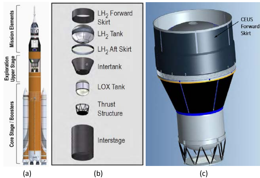
Figure 1. Schematics of (a) the SLS Block 1B configuration, showing the location of the Exploration Upper Stage 7 , (b) an exploded view of the Exploration Upper Stage 6 , and (c) an assembled view of the Exploration Upper Stage, showing the forward skirt location 6 .
