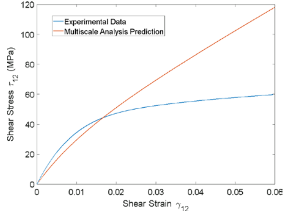
Figure 18. Level 2 prediction of nonlinear shear stress-strain response of AS4/GNP/EPON862 with 56% AS4 volume fraction and 1.15% GNP volume fraction in the EPON862 matrix.
