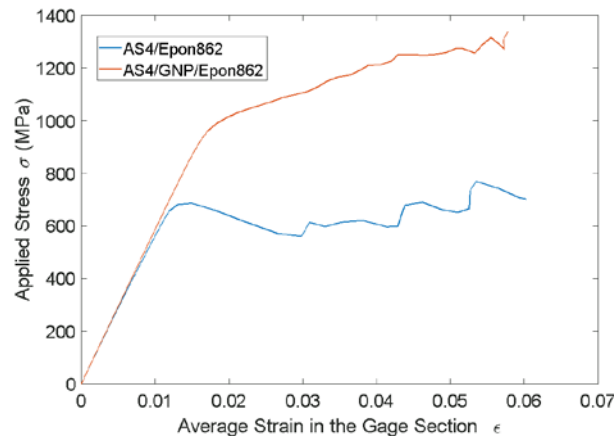
Figure 22. Applied compressive stress versus average compressive strain in gage section of OHC cross-ply specimen for AS4/EPON862 system with 56% volume fraction of AS4 and AS4/C-300/EPON862 system with 56% volume fraction of AS4 and 1.21% volume fraction of GNP within EPON862 matrix.
