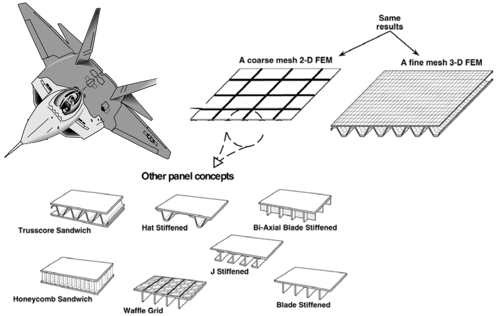
Figure 8. HyperSizer’s approach is to generate FEM properties for shell finite elements using a planar, 2-D coarse mesh that permits the FEA solver to compute internal loads as accurately as accomplished with finely meshed 3-D discrete models. This allows the design-by-analysis process to determine the best panel design for all vehicle locations, using the same loads model mesh.
