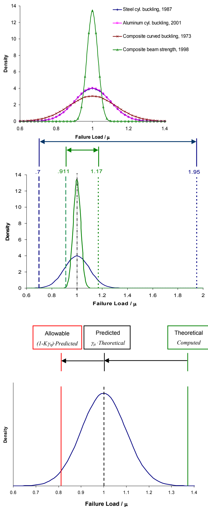
Figure 4a, 4b, and 4c. PDF plots normalized to (failure load/ \mu ), where \mu is the mean failure load.
