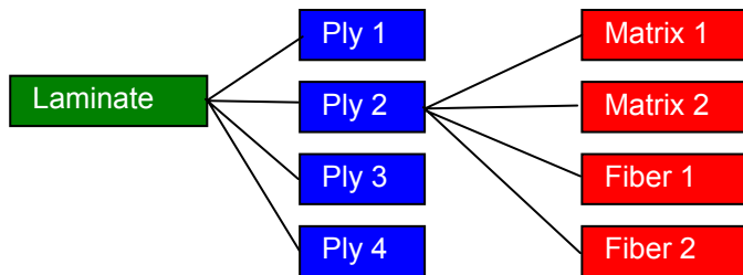
Figure 1: Material linking in HyperSizer
